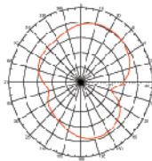
H-Plane at 2.5 GHz
