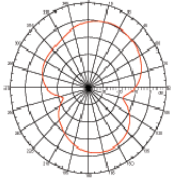
H-Plane at 2.4 GHz
