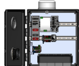
UPS Integrated System with SLA Batteries, NEMA 3R Poly Enclosure, 480 W Power, & Cisco IR1101 SKU 201993 MFG PART #: VP-148D1-07111-3
