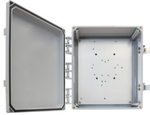
12x10x6 Enclosure with Solid Door, Latch Locks, Cisco Backplate Tessco No 540559
